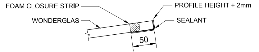
SECTION - A
